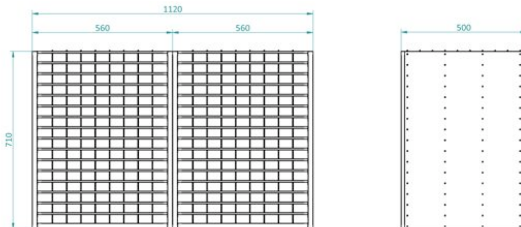
Dimensions of the Honeycomb system, item number 20050101
