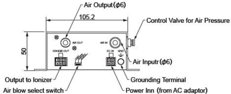
Controler Unit
